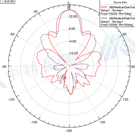
Radiation Pattern 9
