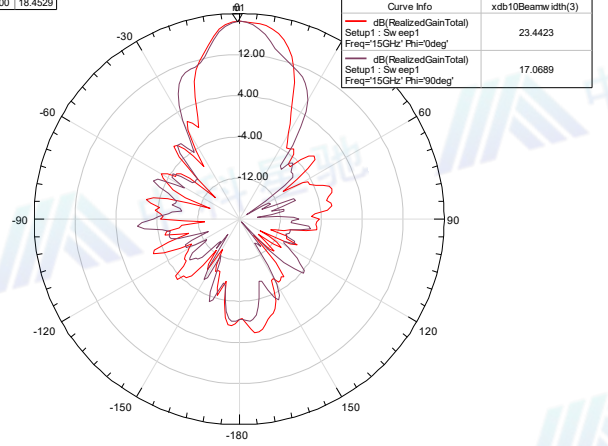
Radiation Pattern 14
