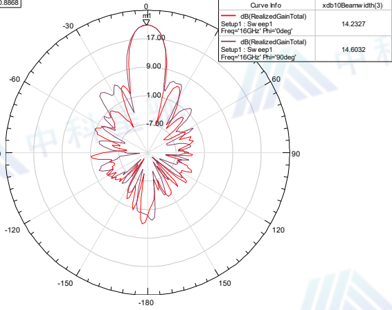
Radiation Pattern 15
