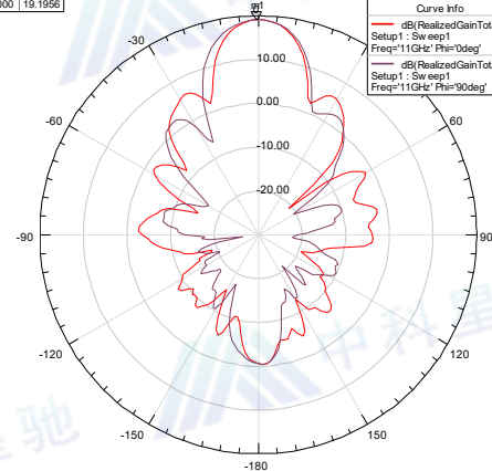
Radiation Pattern 10
