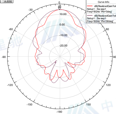
Radiation Pattern 7
