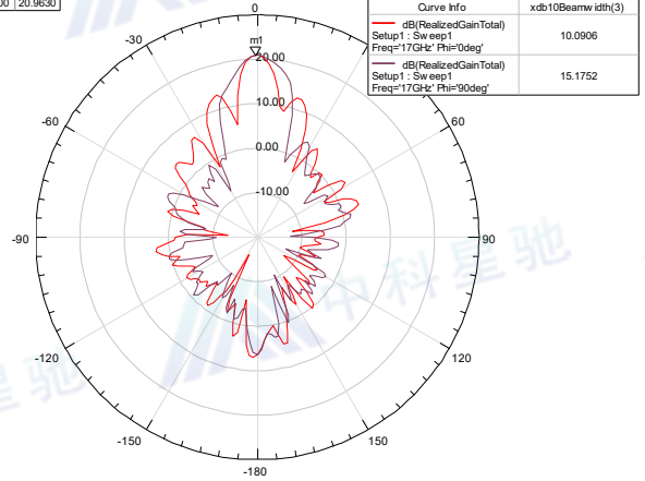
Radiation Pattern 16
