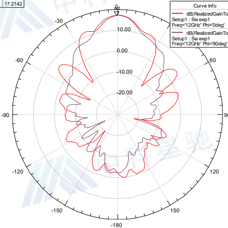
Radiation Pattern 11
