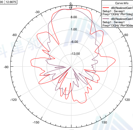
Radiation Pattern 12
