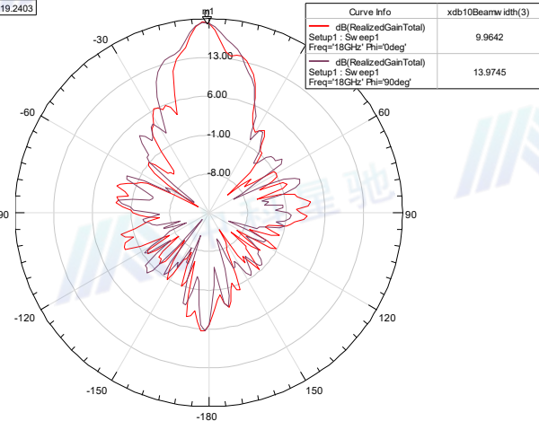
Radiation Pattern 17
