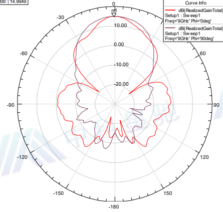
Radiation Pattern 8
